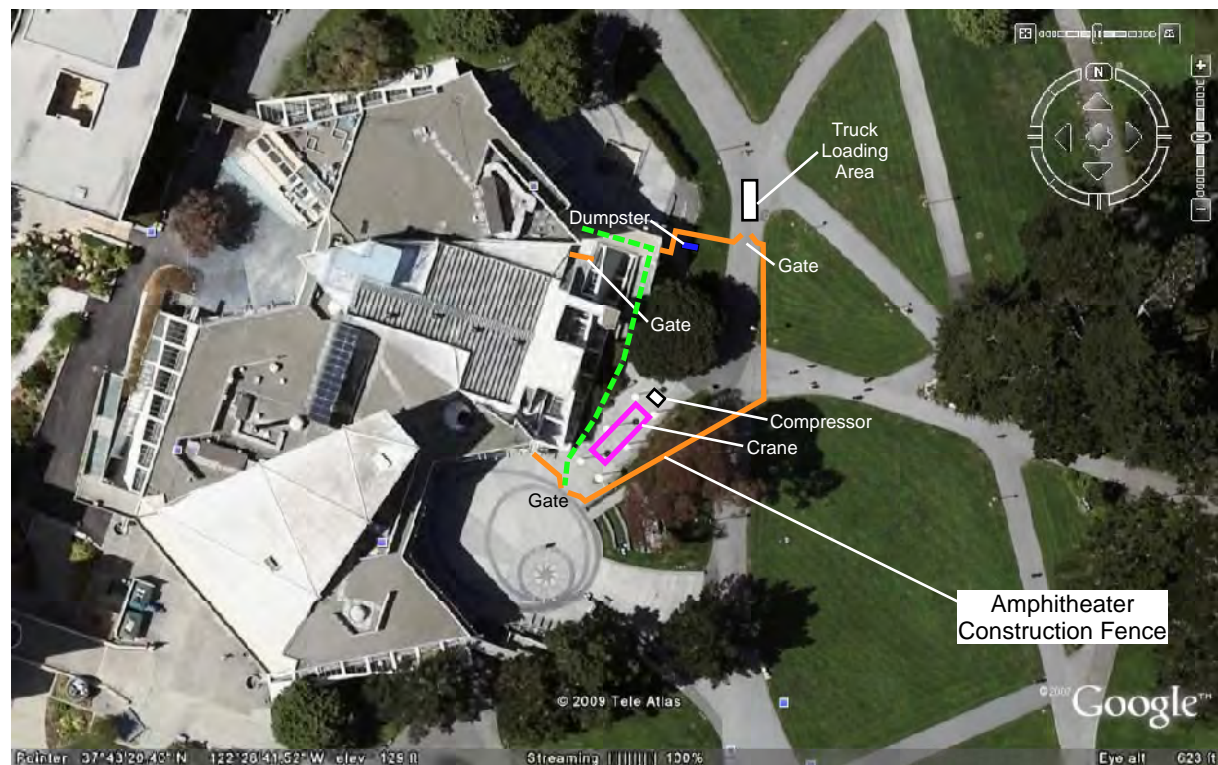
Amphitheater Site Plan
